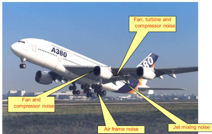
figure 6 Overview of the noise sources of a modern jet aircraft (see Chapter 14 for more information).
