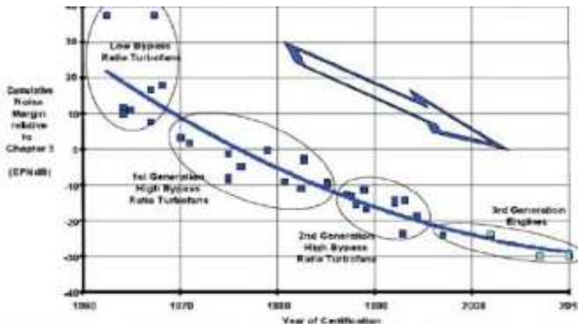
figure 25 The trend towards lower noise aircraft closely follows the increasing by-pass ratios.
